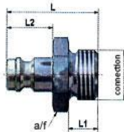
Plug, male
