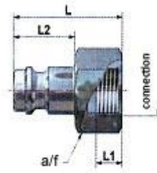
Plug, female
